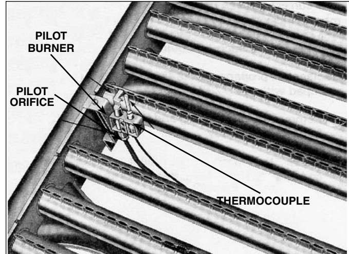
Figure 4.3 Pilot
