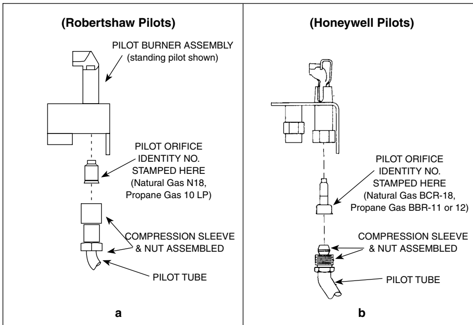
Figure 4.2 Pilot Orifices
